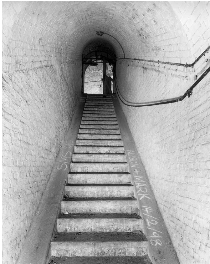
Figure 23 Steps leading up from the gun rooms to the road tunnel; note the wheeling ramps on either side to enable heavy guns to be moved easily (NMR: AA/009830)
