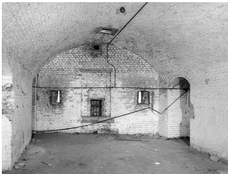
Figure 24 No 2 gun room, showing the central carronade embrasure flanked by two musket loopholes (NMR: AA00/9831)
