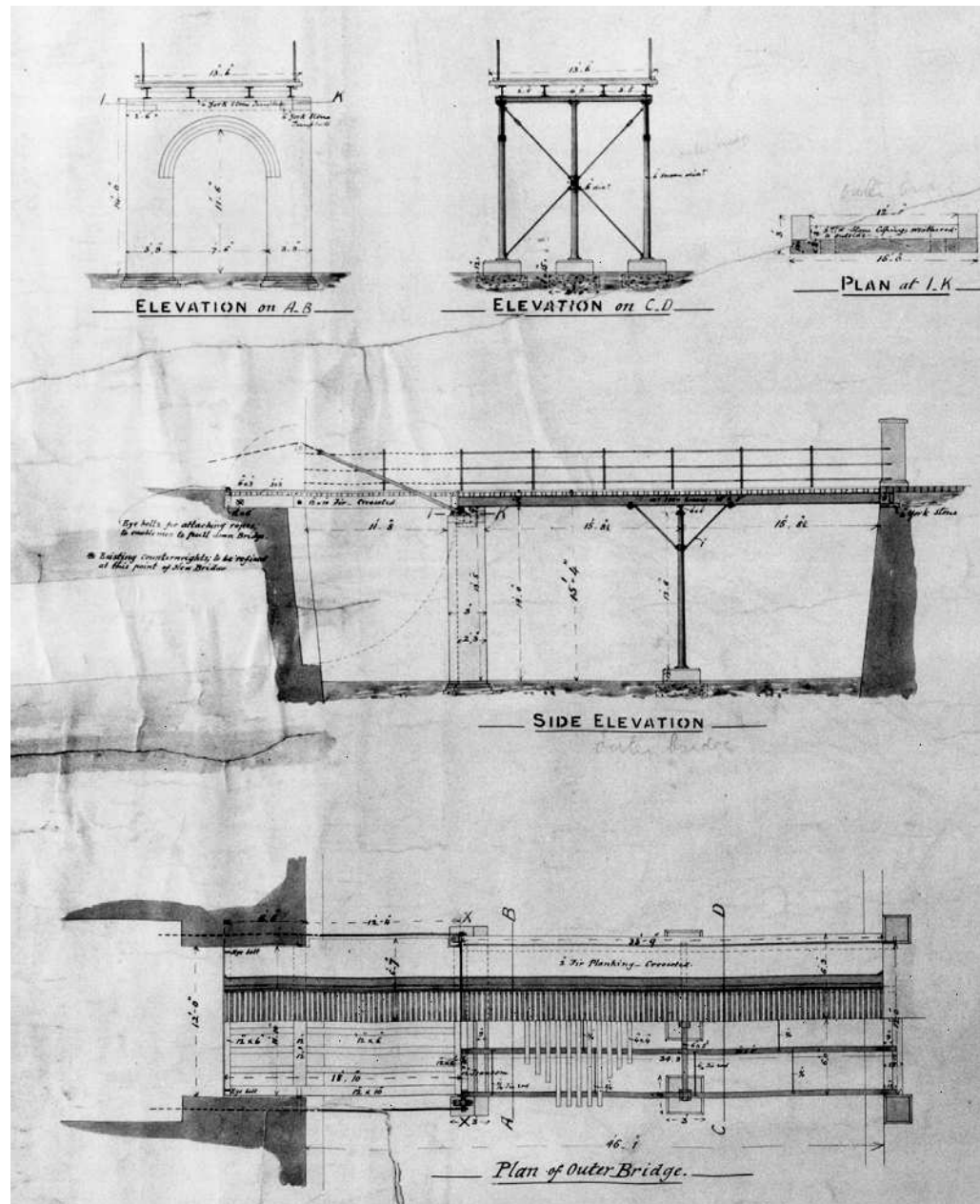
Figure 12 A plan dated 1887, showing the proposed new bridges at the North Entrance (extract from NMR: WD/2315)
