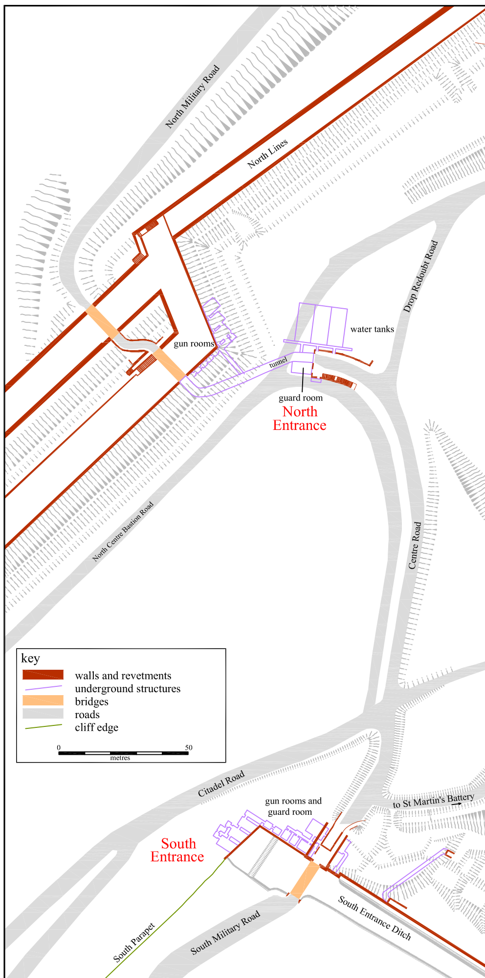
Figure 8 Plan showing the North and South Entrances following the 1860s remodelling
