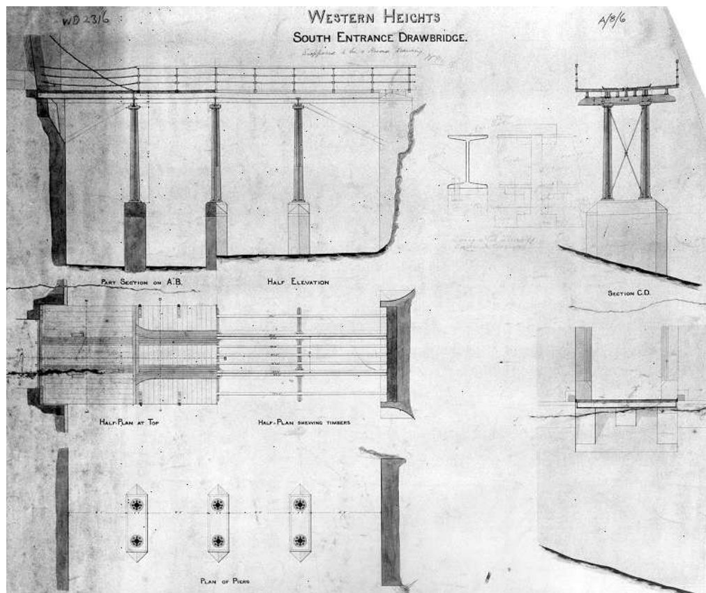
Figure 34 A plan dated 1876, showing the bridge at the South Entrance (NMR: WD/2316)
