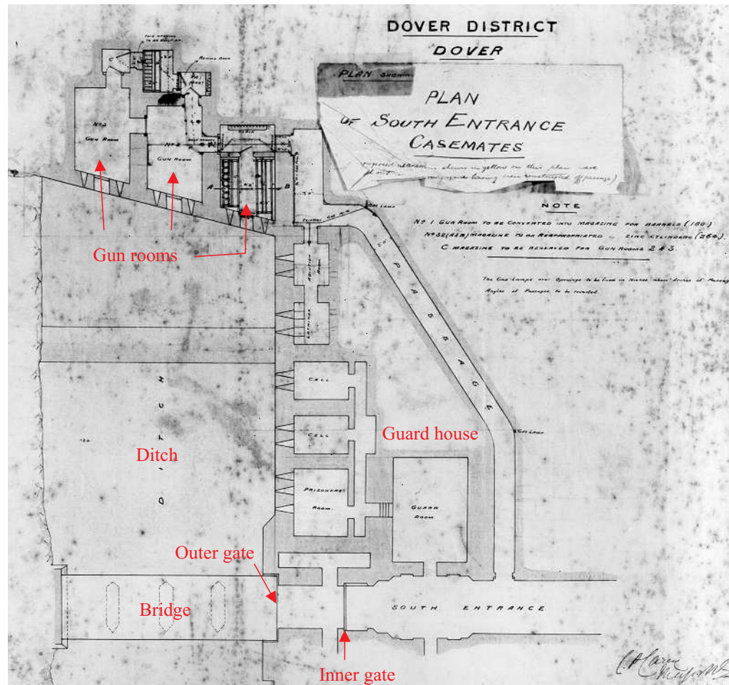
Figure 36 A plan dated 1876 of the South Entrance. Text in red is added by the authors (NMR: WD/2358)
