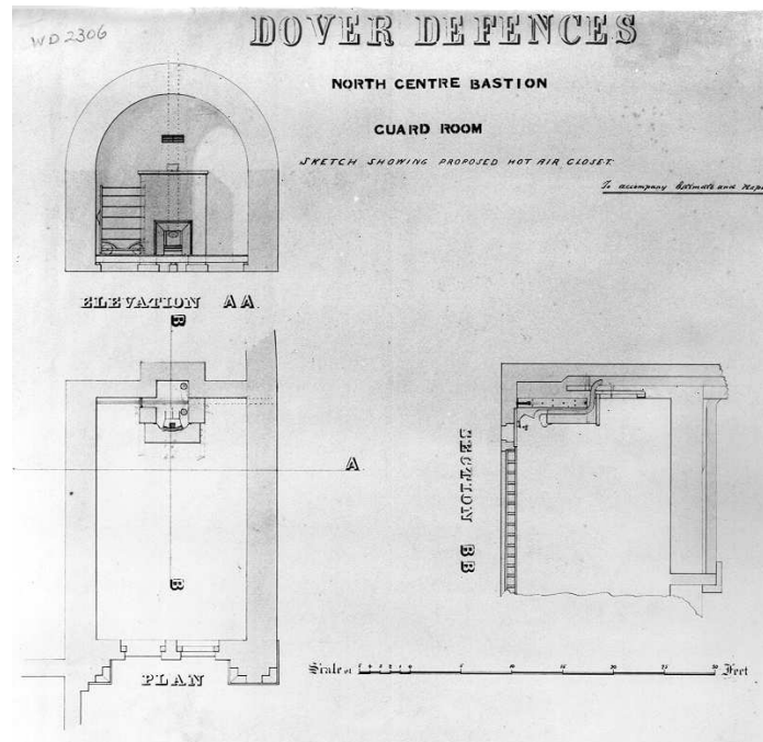
Figure 28 A plan dated 1861 showing details of the hot air closet inserted into the guard house (NMR: WD/2306)
