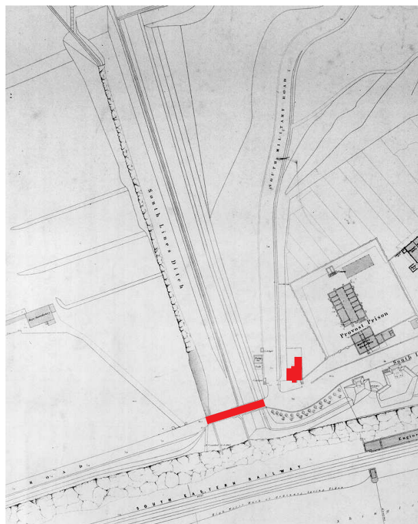
Figure 4 The South Lines in 1893, showing the South Lines Bridge, one of the original entrances into the Fortress. The bridge and the nearby piquet house are shown with red added by the authors (extract from NMR: WD/2396)
