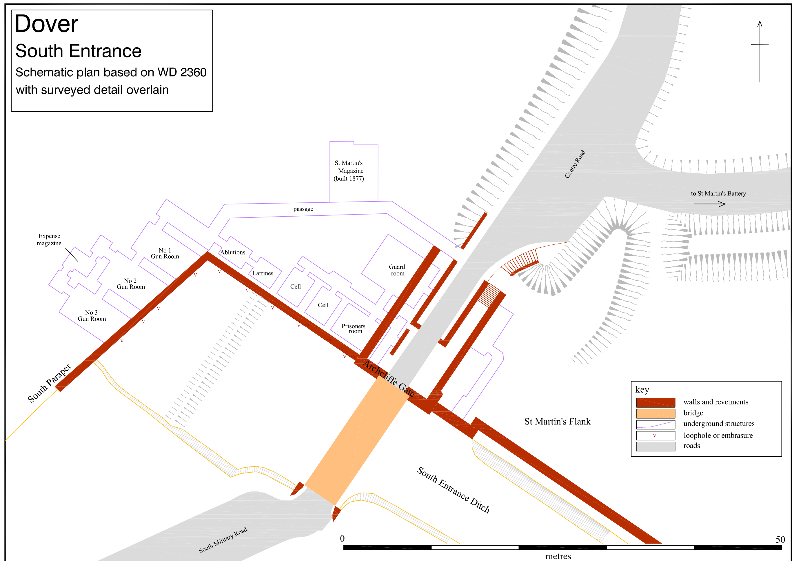
Figure 31 A plan of the South Entrance, based upon a plan dated 1876
