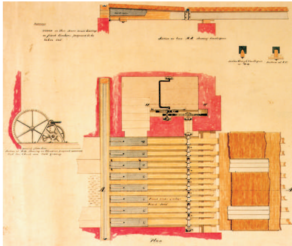
Figure 19 A plan dated 1863, showing part of the inner bridge and its counterpoise weights and lifting gear (extract from NMR: WD/2308)
