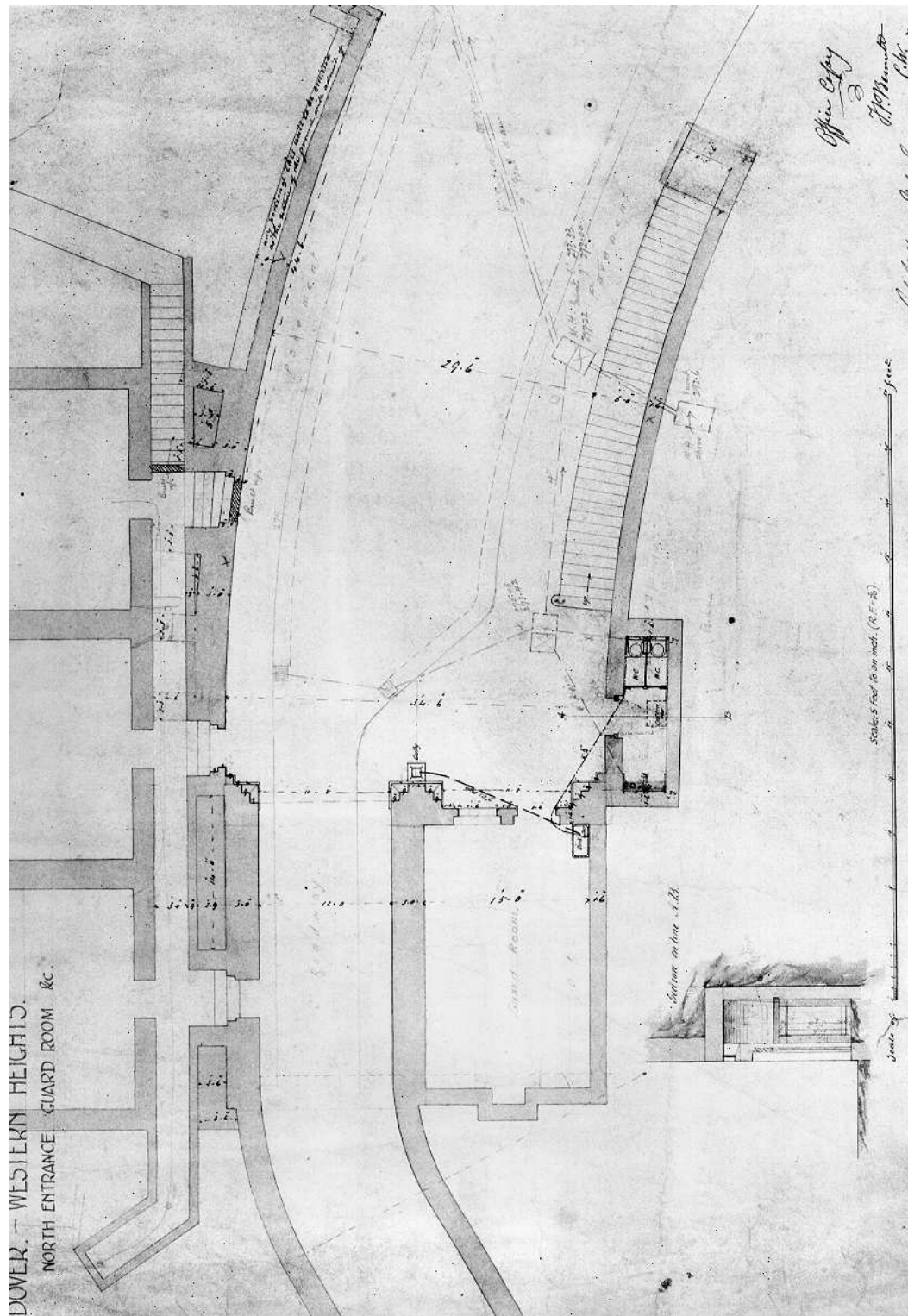
Figure 26 A plan of the Inner Entrance, dated 1861 (NMR: WD/2305)
