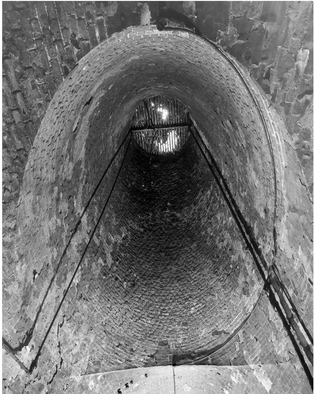
Figure 22 The vertical elliptical opening in the roof of the road tunnel (NMR: AA00/9827)
