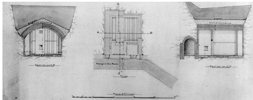
Figure 38 A plan dated 1878, of the new magazine for St Martin's Battery (NMR: WD/2360)
