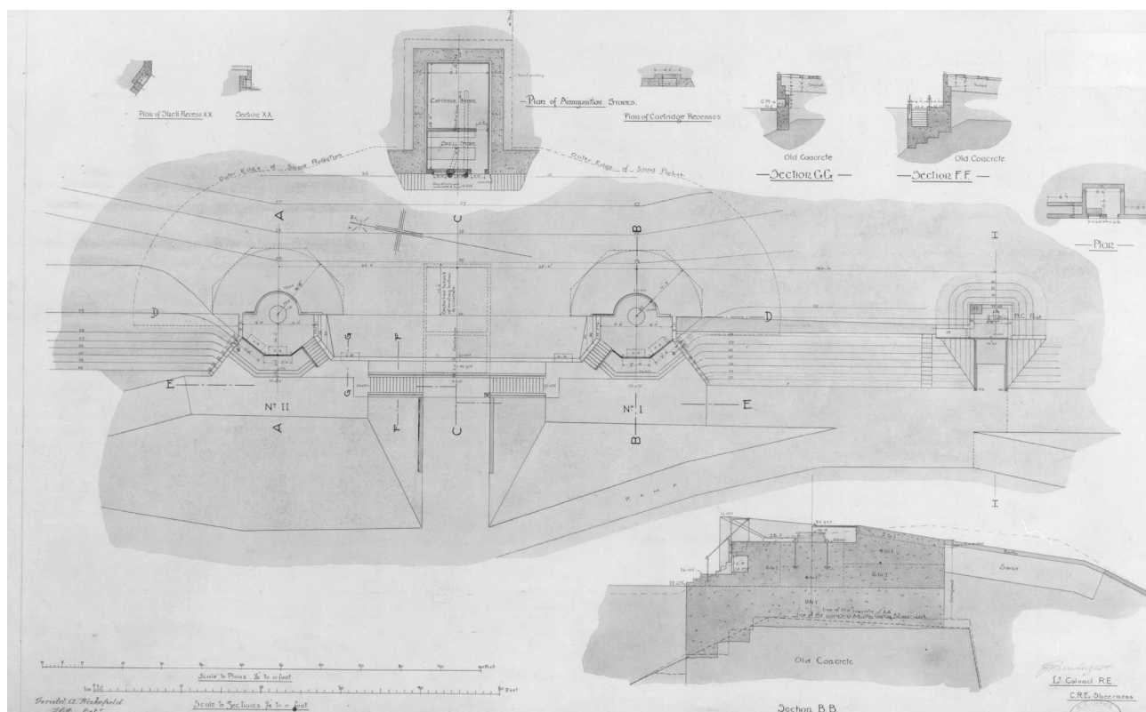
Figure 27 Plan dated 1906 of the new 4.7-inch QF battery (PRO: WO/78/5115/3)
