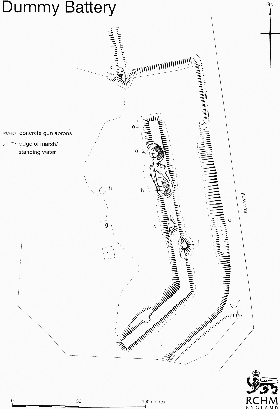
Figure 28 RCHME survey plan of Dummy Battery.
