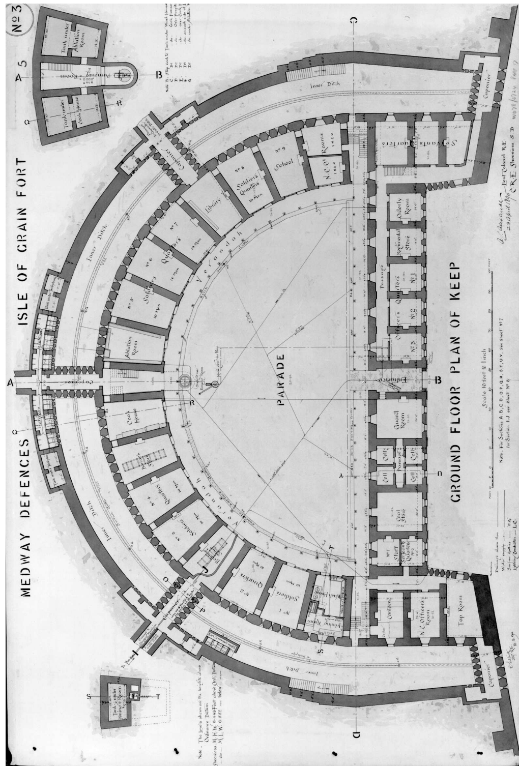
Figure 24 Plan dated 1895 of the ground floor of the keep (PRO: WO/78/5124/17)
