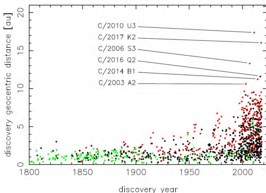
Geocentric discovery distances for all 1065 long-period comets (LPCs) versus discovery date [reference: Discovery statistics and the 1/a-distribution of long-period comets detected over the 1801–2017 period. Małgorzata Królikowska, Piotr A Dybczynski, Monthly Notices of the Royal Astronomical Society, Volume 484, Issue 3, 11 April 2019, Pages 3463–3475, open publication: arxiv.org/abs/1901.01722 ].
